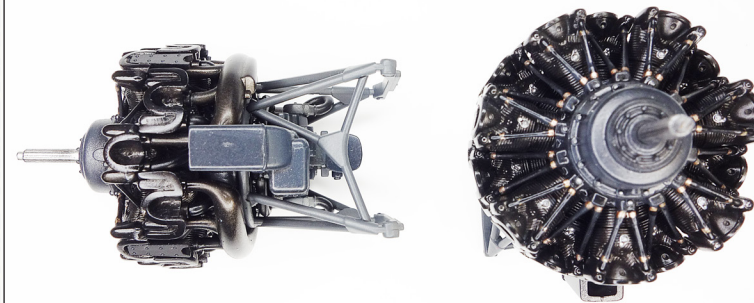
底面と前方写真 / Bottom View and Front Side View
