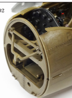
キ45改丙(陸軍航空工廠製) Ki-45 Kai Hei (Manufactured in the Army Aerial Arsenal)
