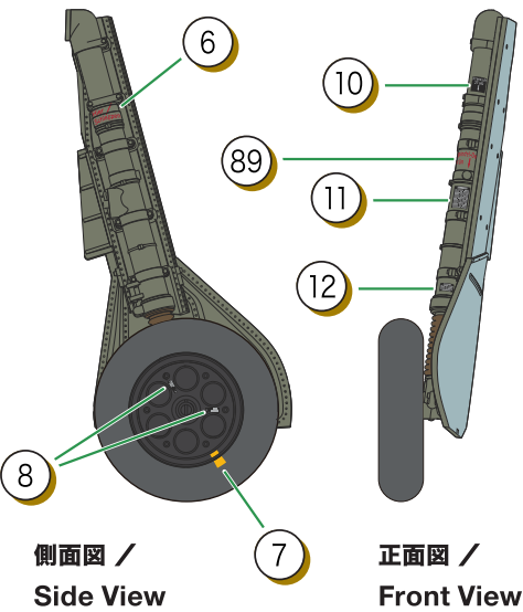
主脚(左側) Main Landing Gear (Left side)
