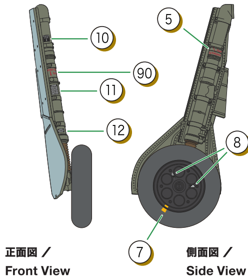
主脚(右側) Main Landing Gear (Right side)
