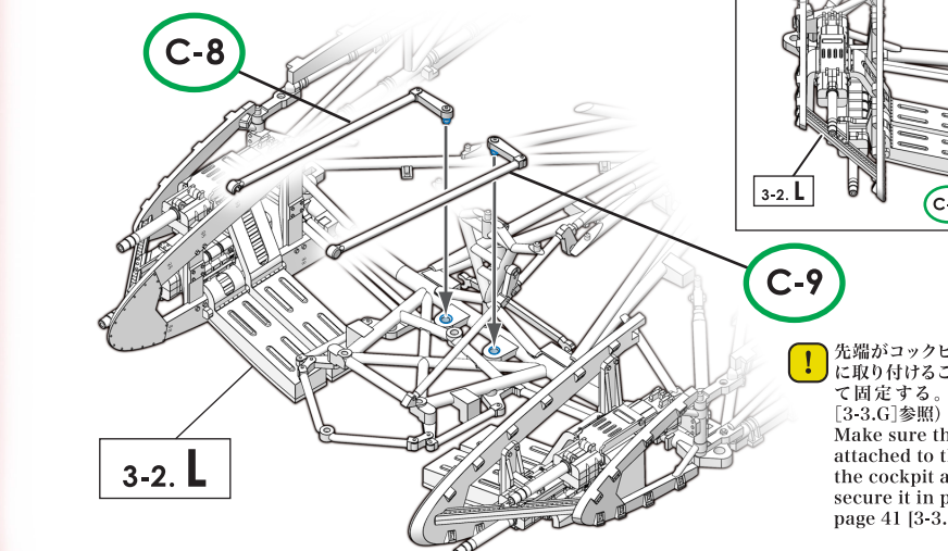
各パーツ接着位置 Parts configuration after assembly.
