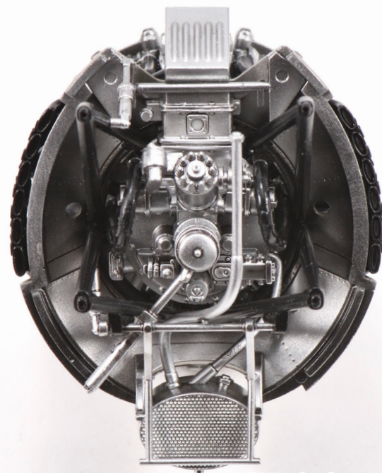
背面写真 / Rear View
